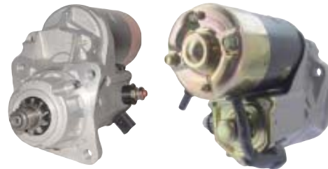
17388* 12V, 2.5kw, CW, 10-Tooth Denso OSGR, Heavy Duty
