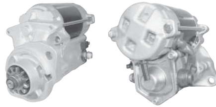
17619 12V, 4.8kw, CW, 11-Tooth Denso OSGR, Waffle Type
