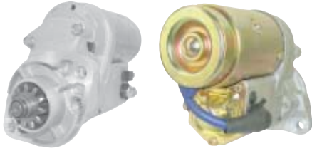
17116 12V, 1.4kw, CW, 11-Tooth Denso OSGR, Gold Case
