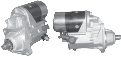
16658 12V, 2.5kw, CW, 10-Tooth Denso OSGR, Heavy Duty
