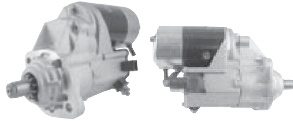
17362 12V, 2.5kw CW, 11-Tooth Denso OSGR, Heavy Duty
