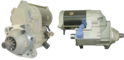
18458 24V, 7.8kw, CW, 11-Tooth Denso OSGR, Heavy Duty
