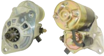
17292 12V, 2.5kw, CW, 11-Tooth Denso OSGR, Heavy Duty
