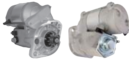
18142 12V, 1.4kw CW, 11-Tooth Denso OSGR, Silver Type
